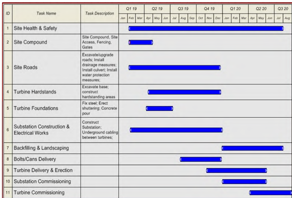
Figure 8.1 Indicative Construction Schedule
